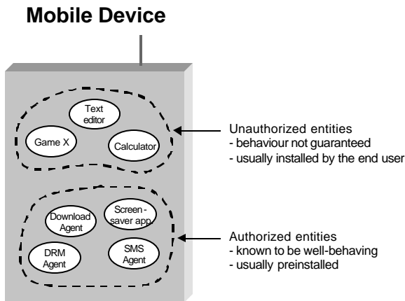
Figure 4. Authorized and unauthorized entities
