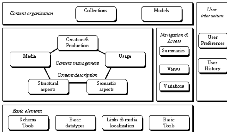
Figure 3 - Overview of MPEG-7 Multimedia DSs [16]
