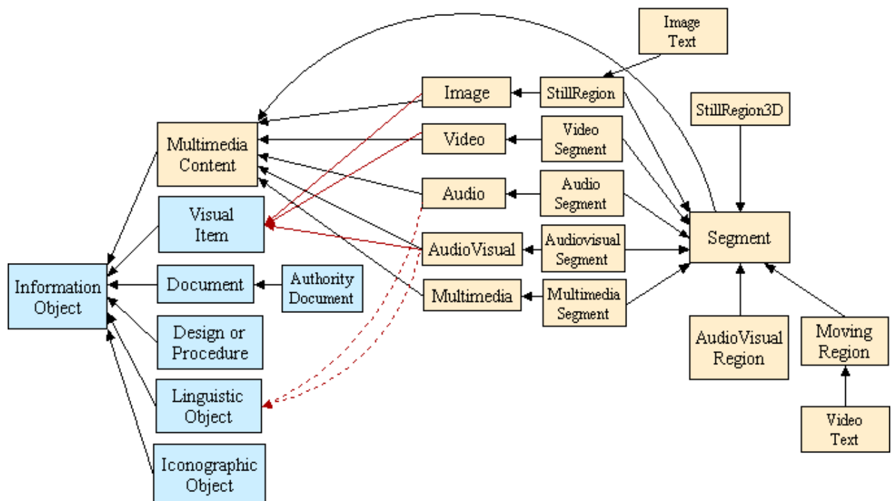
Figure 4 - Extending the CIDOC CRM Class Hierarchy with MPEG-7 Multimedia Subclasses
