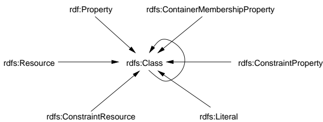
Figure 3. The instance-of relationships of modeling primitives in RDFS.
